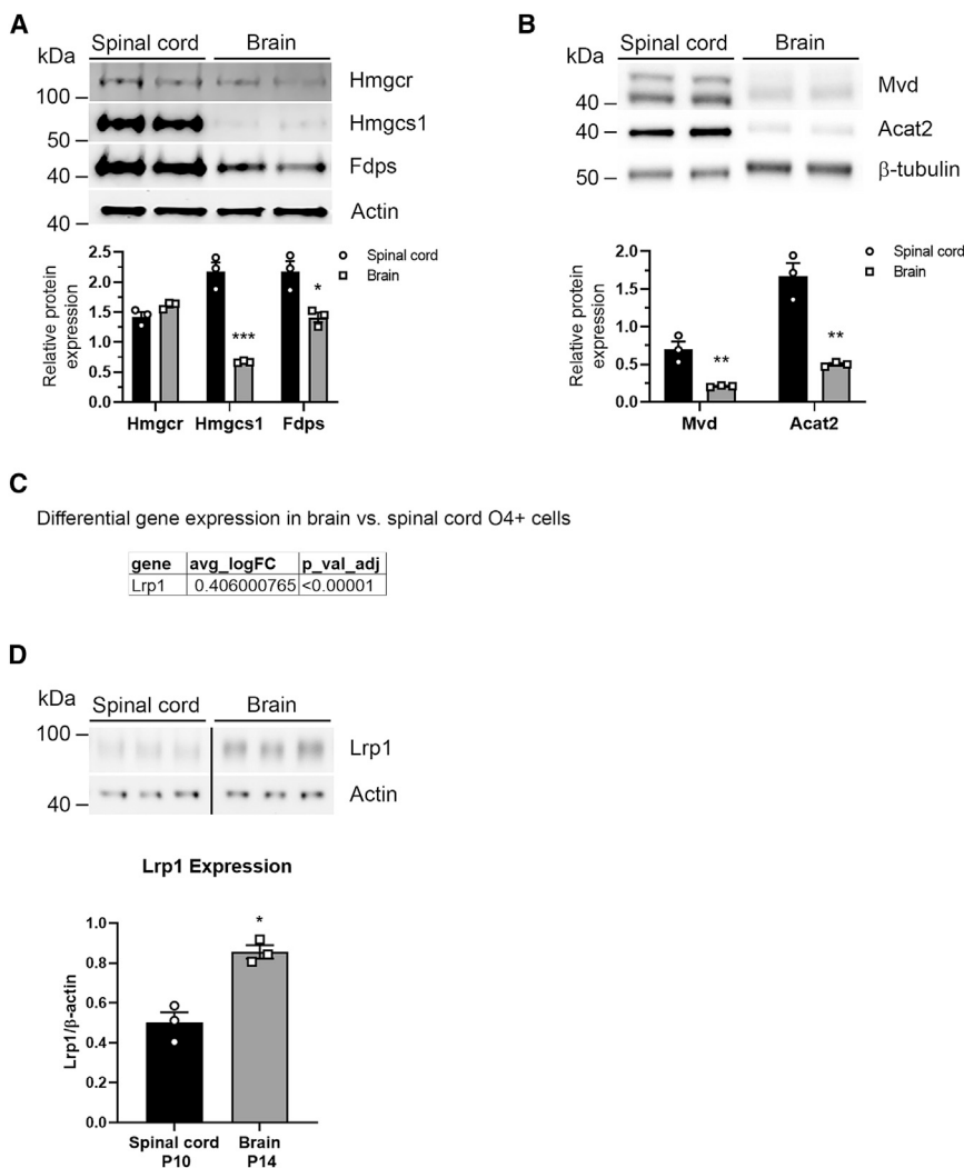
Figure 2. Brain and spinal cord oligodendroglia have different dependence on cholesterol synthesis and uptake
