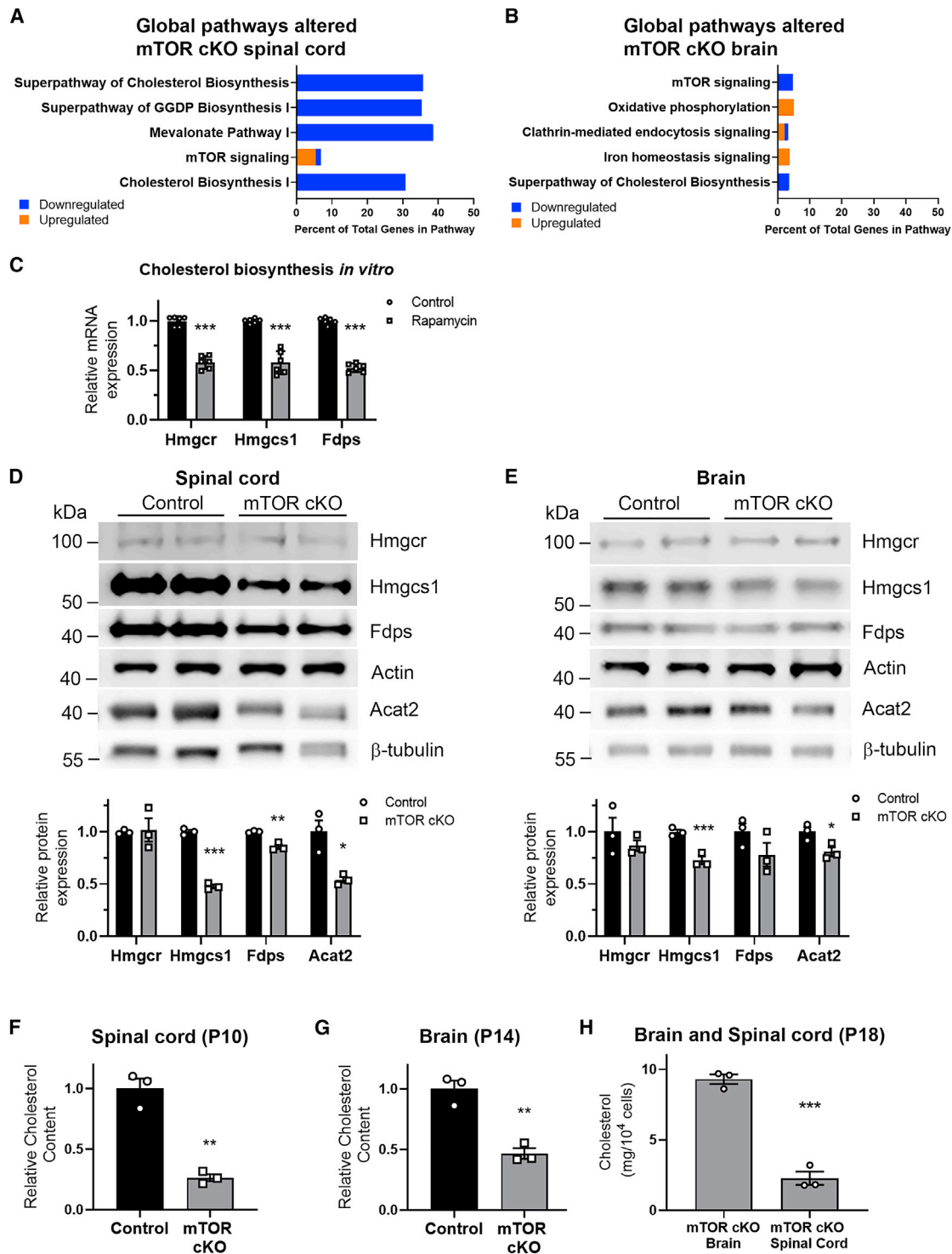
Figure 4. mTOR is necessary for normal cholesterol biosynthesis in oligodendroglia
